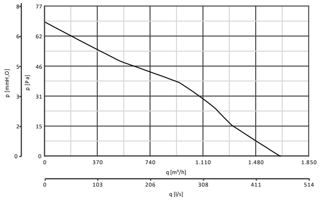
VORTICE 300/12" AR LL S cod 12415
