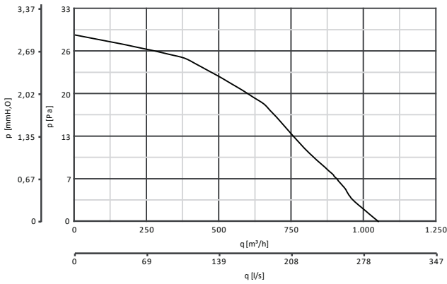
VORTICE 300/12" AR cod 12412
