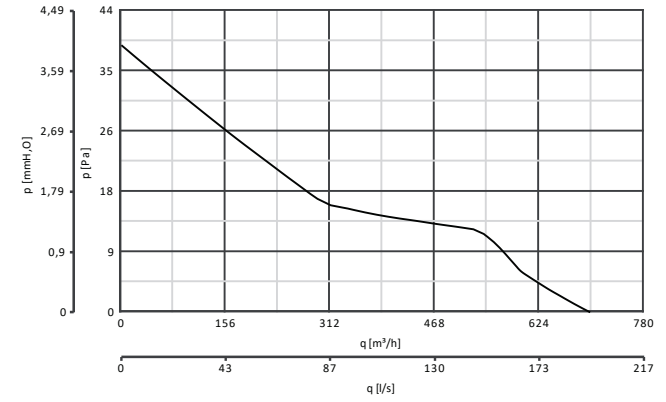
VORTICE 230/9" ARI LL S cod 12456
