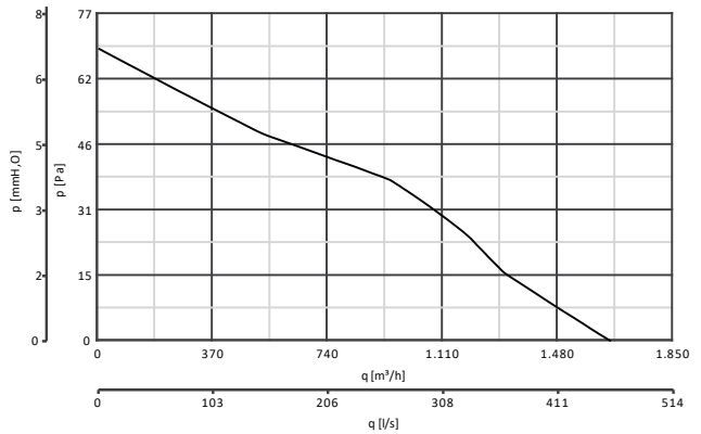
VORTICE 300/12" ARI LL S cod 12416
