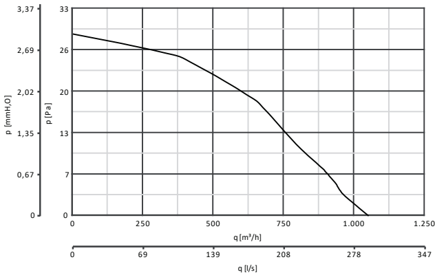
VORTICE 300/12" ARI cod 12413
