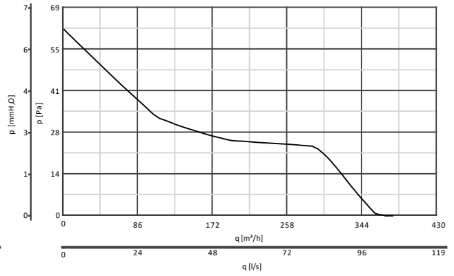
VORTICE 150/6" ARI LL S cod 12616
